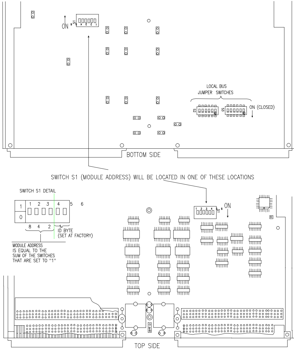
Figure 1-3, Local Bus Jumper Switches and Module Address Switches
